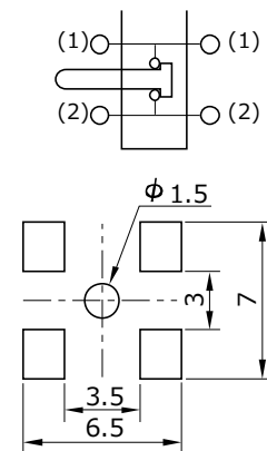
P. C. Board Dimension
