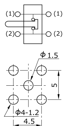
P. C. Board Dimension
