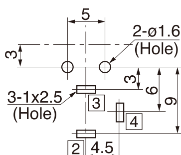
Recommended PCB Layout (Pattern Side) / Compatible Plug
