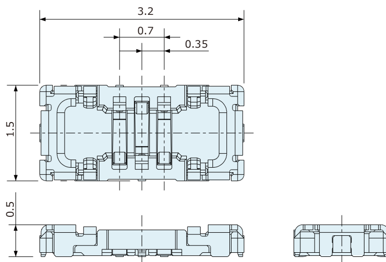
Socket:CPBE305-0101F
