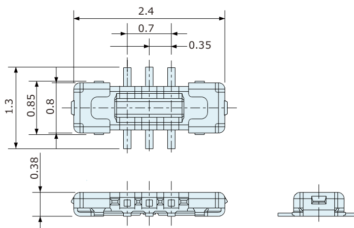
Plug:CPBE405-0101F
