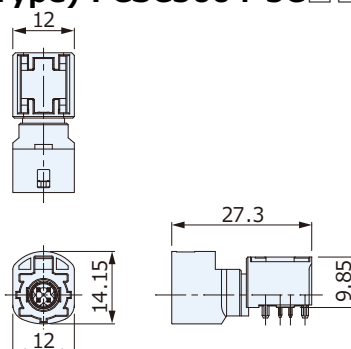
Plug(Right Angle Type) : CSC5004-5C□□F
