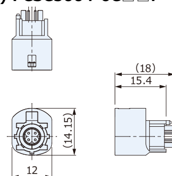
Plug(Vertical Type) : CSC5004-6C□□F
