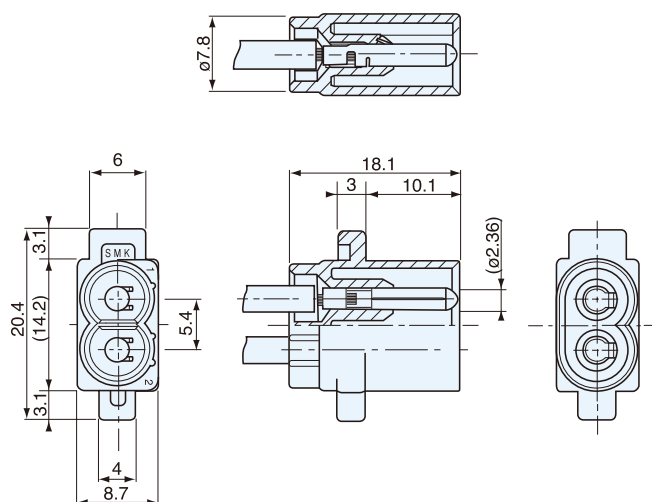
Plug : CCL0105-0100F
