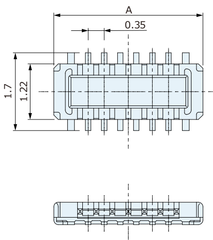
Plug : CPBE8□□-0101F
